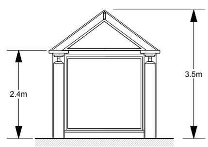
South-East Elevation
