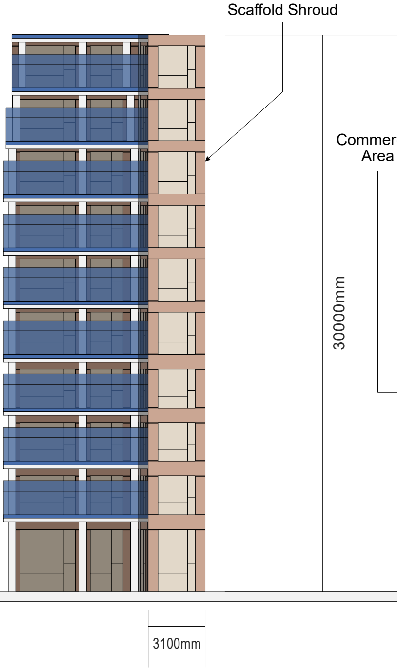
EAST ELEVATION
