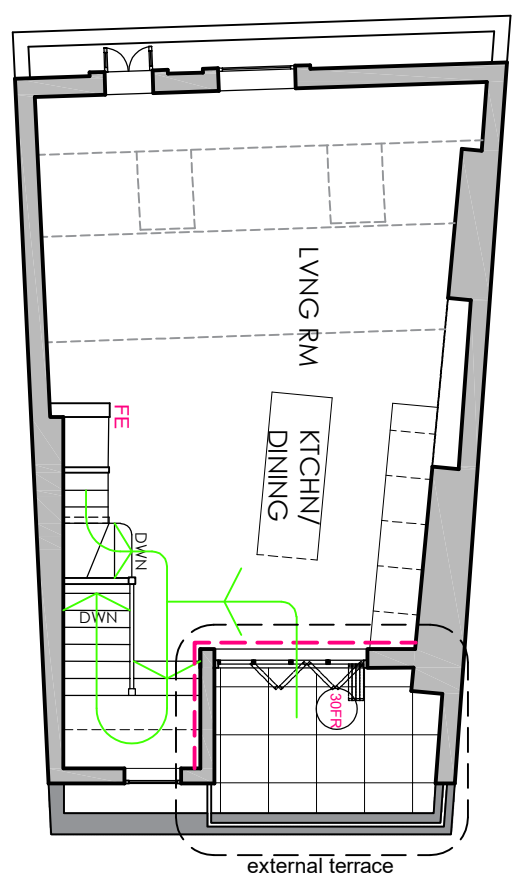
4 THIRD FLOOR
