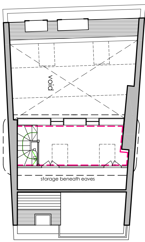
5 MEZZANINE FLOOR
