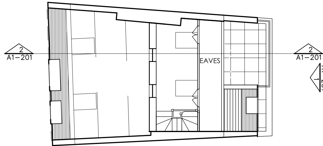
5 MEZZANINE FLOOR
