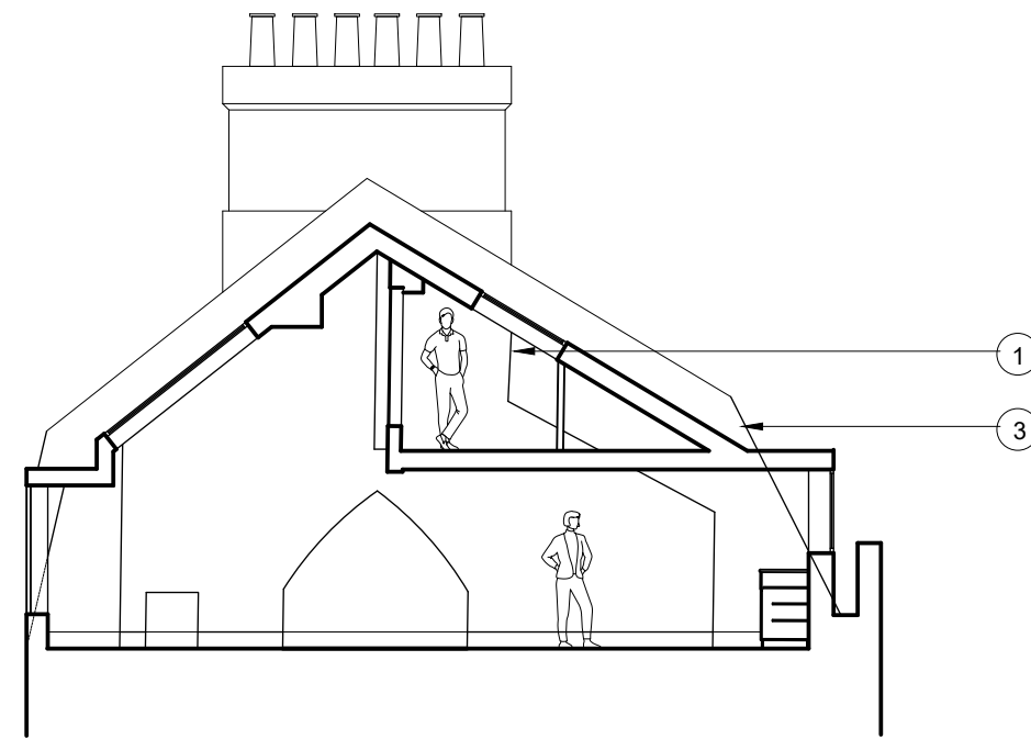
② SECTION
