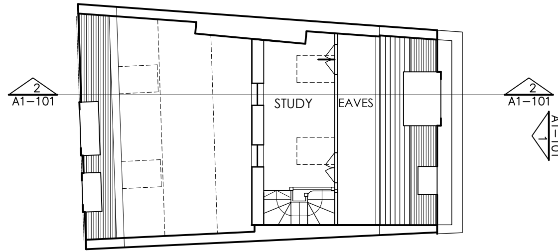
5 MEZZANINE FLOOR
