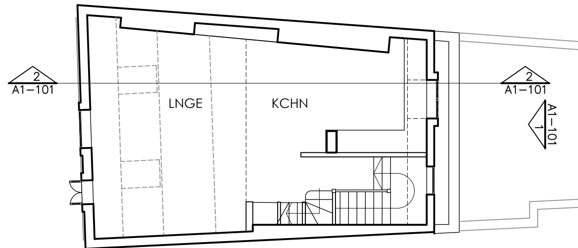
4 THIRD FLOOR
