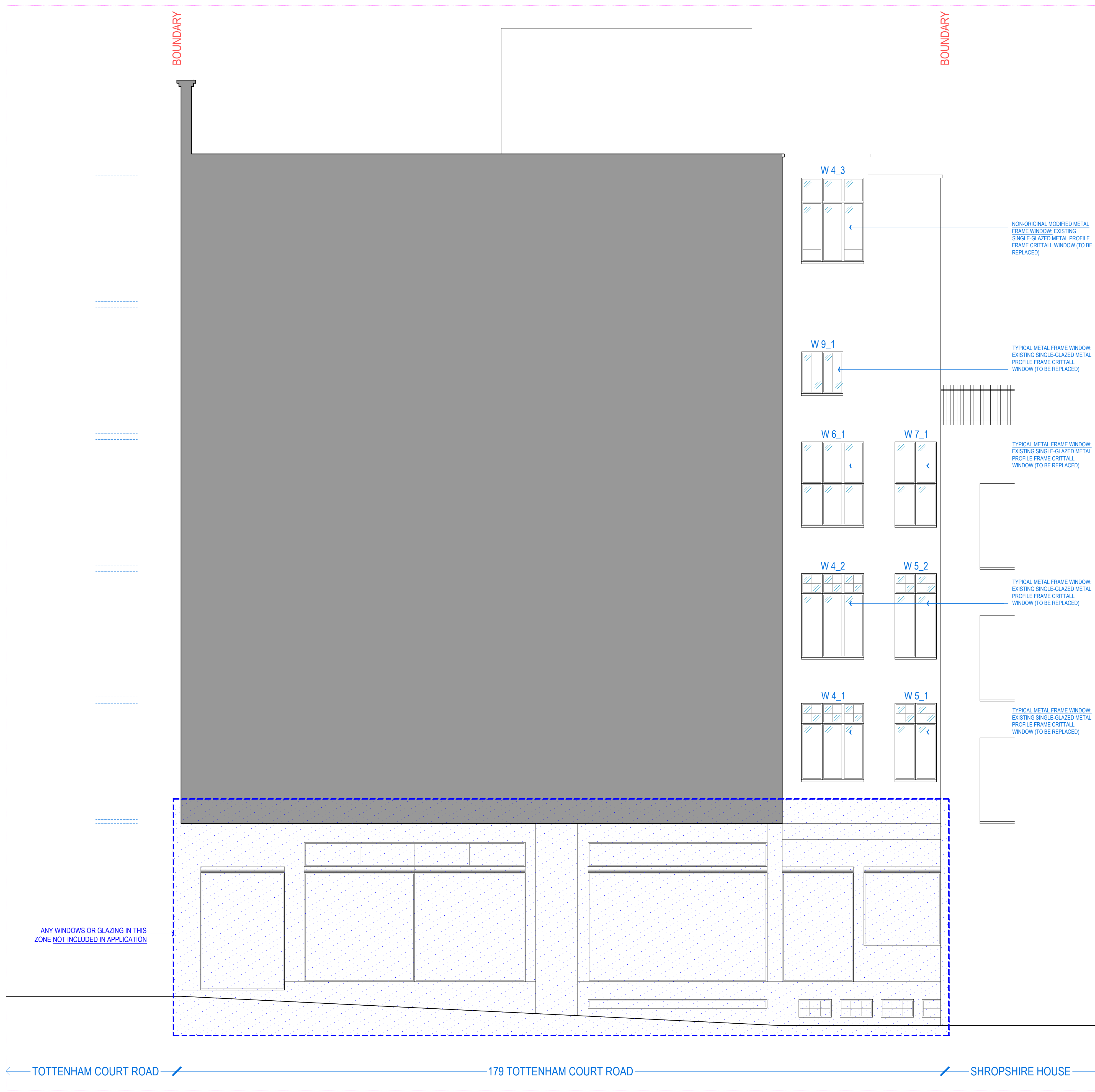
01] EXISTING SECTIONAL ELEVATION
