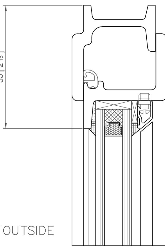
EQUAL SHORT LEG OPTION SHOWN
