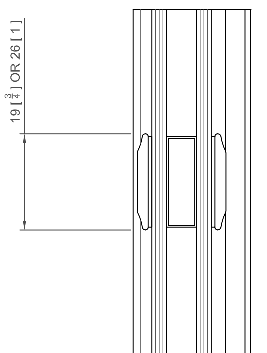
OPTIONAL COSMETIC GLAZING BAR (HERITAGE DUPLEX TYPE)
