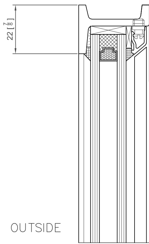
EQUAL SHORT LEG OPTION SHOWN
