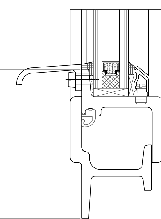
OPTIONAL COSMETIC GLAZING BAR (GRID TYPE)
