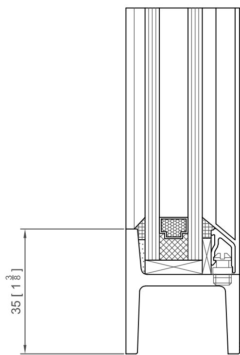
EQUAL LONG LEG OPTION SHOWN
