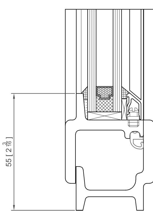
OPTIONAL COSMETIC GLAZING BAR (HERITAGE DUPLEX TYPE)
