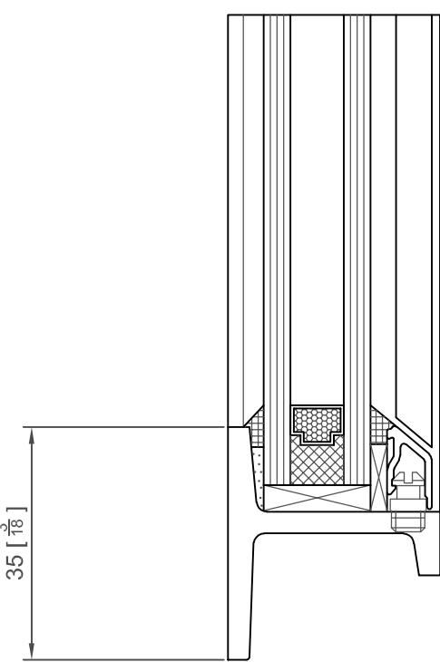
OPTIONAL COSMETIC GLAZING BAR (HERITAGE TYPE)
