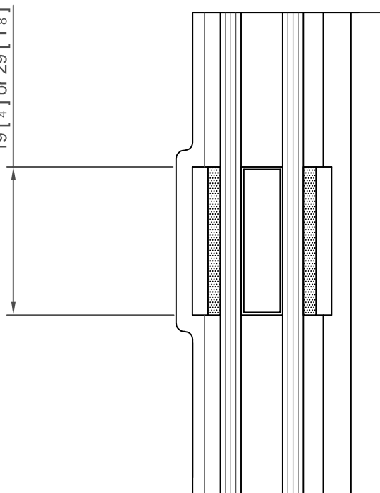
OPTIONAL COSMETIC GLAZING BAR (GRID TYPE)
