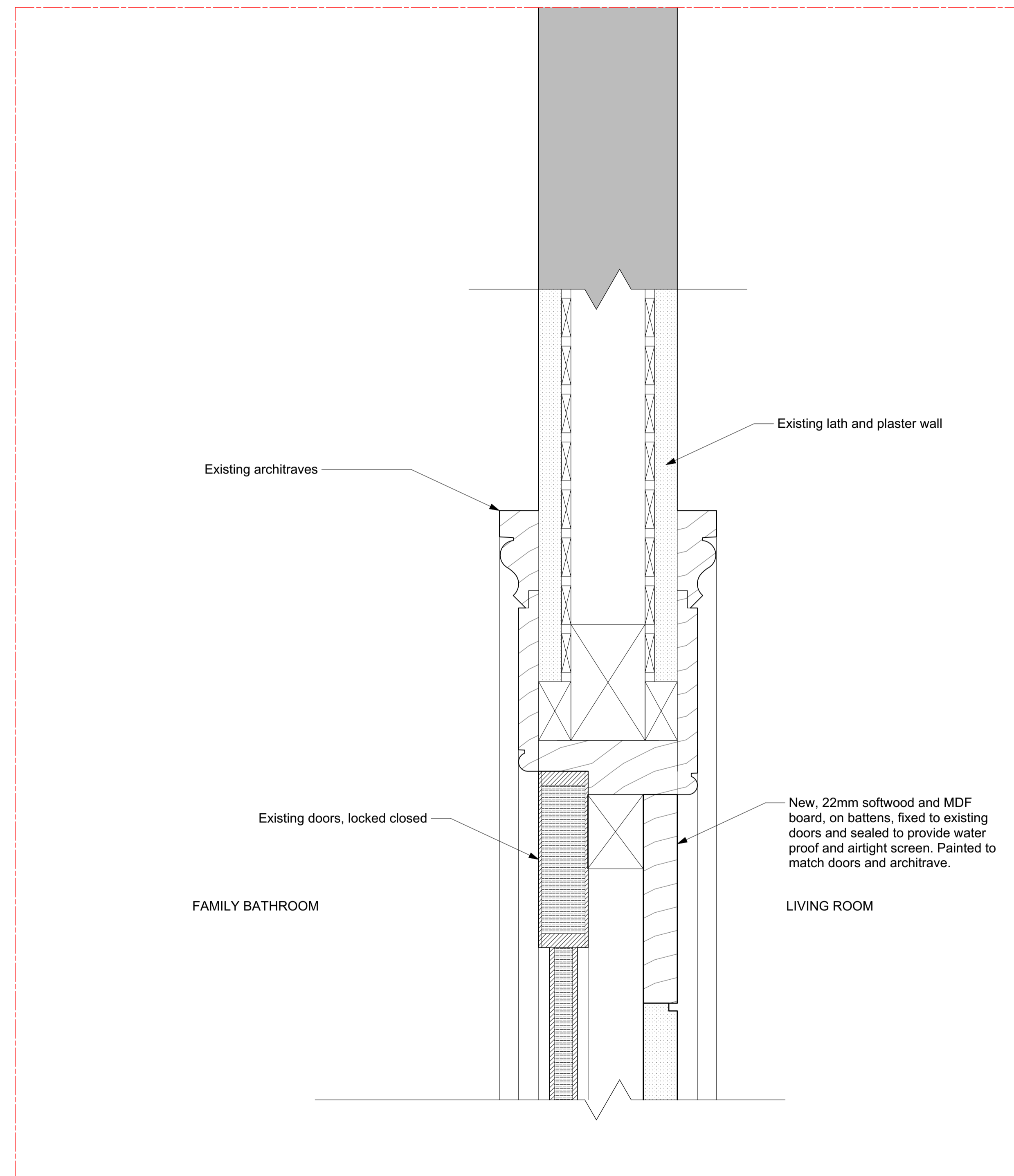
2 First Floor Partition - Detail Section Scale: 1:2
