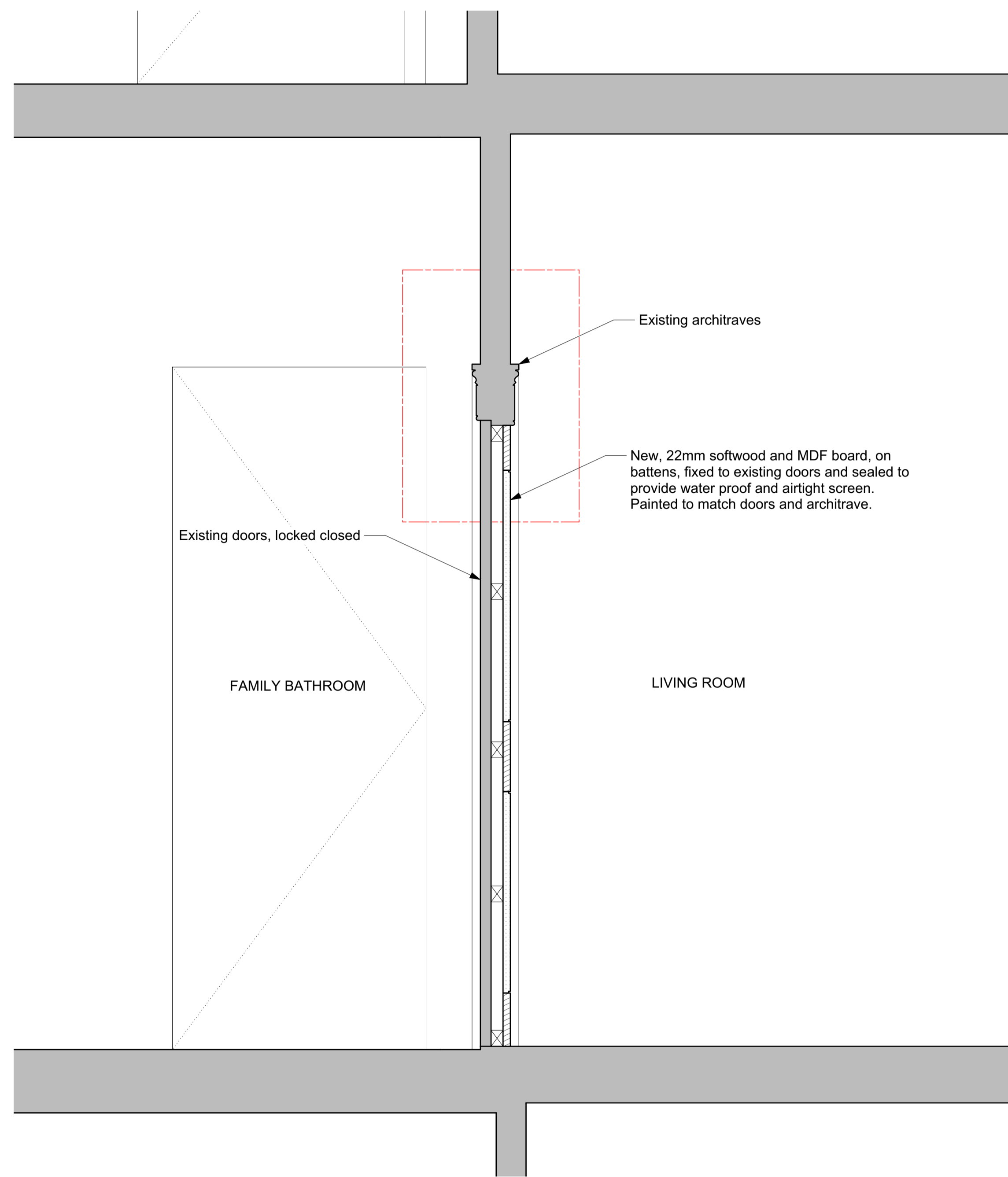
1 First Floor Partition - Section Scale: 1:10
