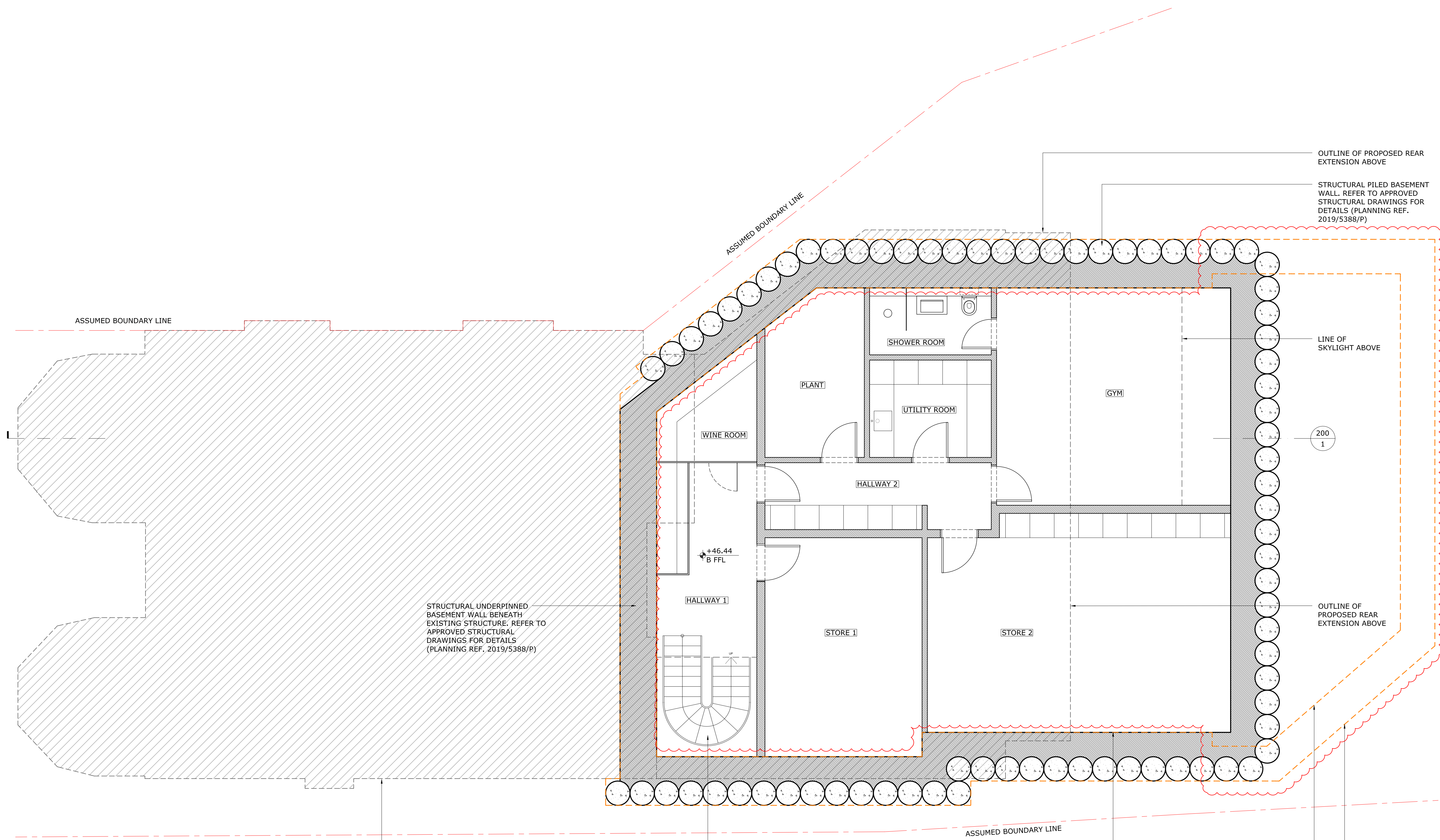
1 PROPOSED BASEMENT FLOOR PLAN 1:50@A1, 1:100@A3
