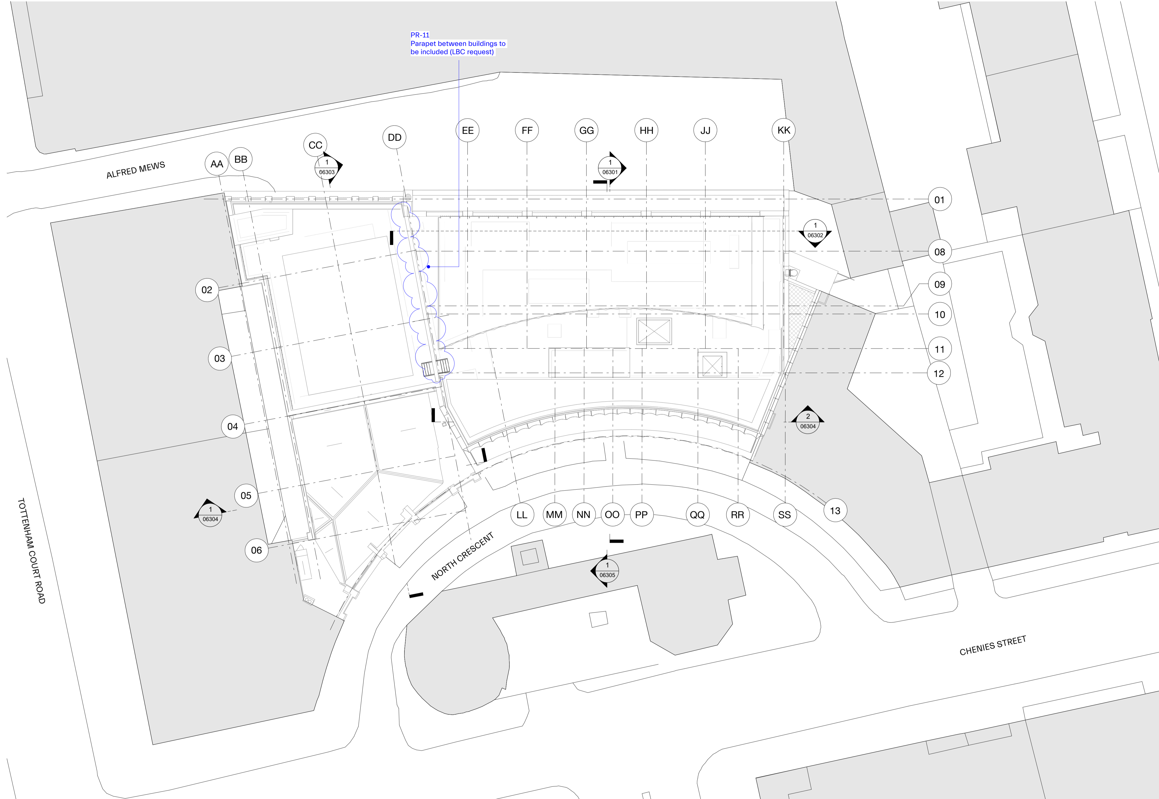
1 06126 PROPOSED ROOF PLAN WITH CONTEXT 1 : 200
