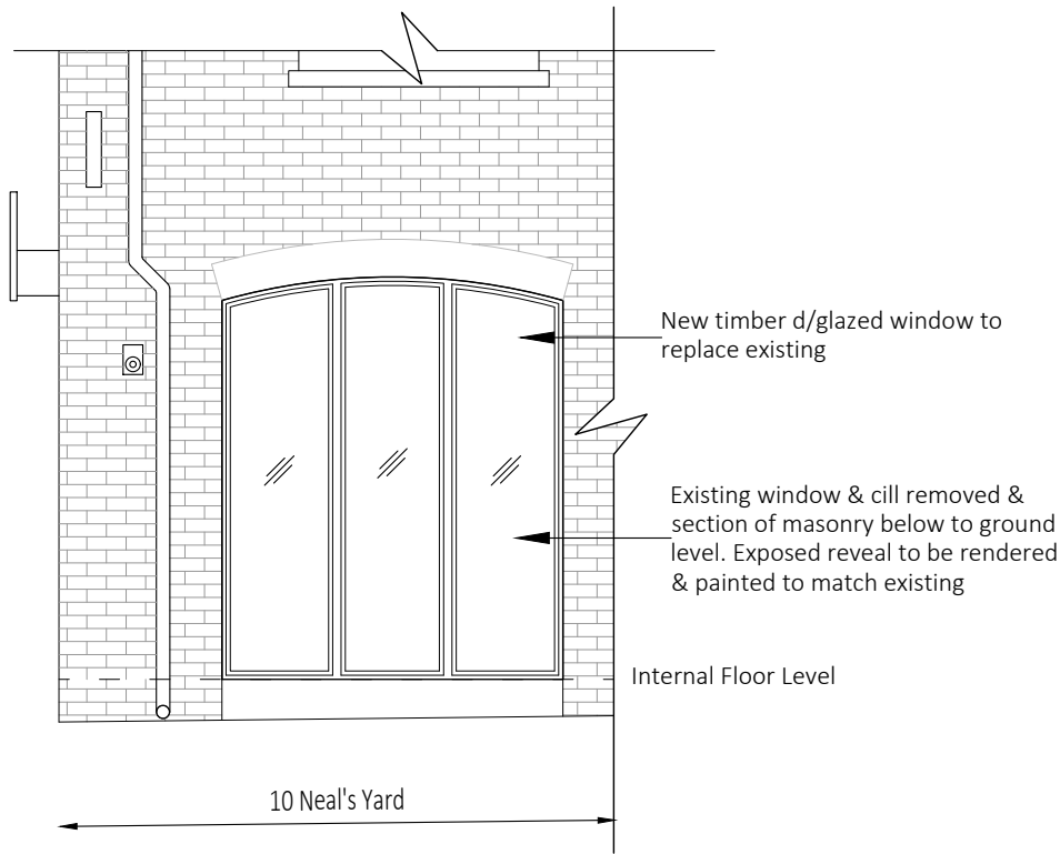
North Elevation
