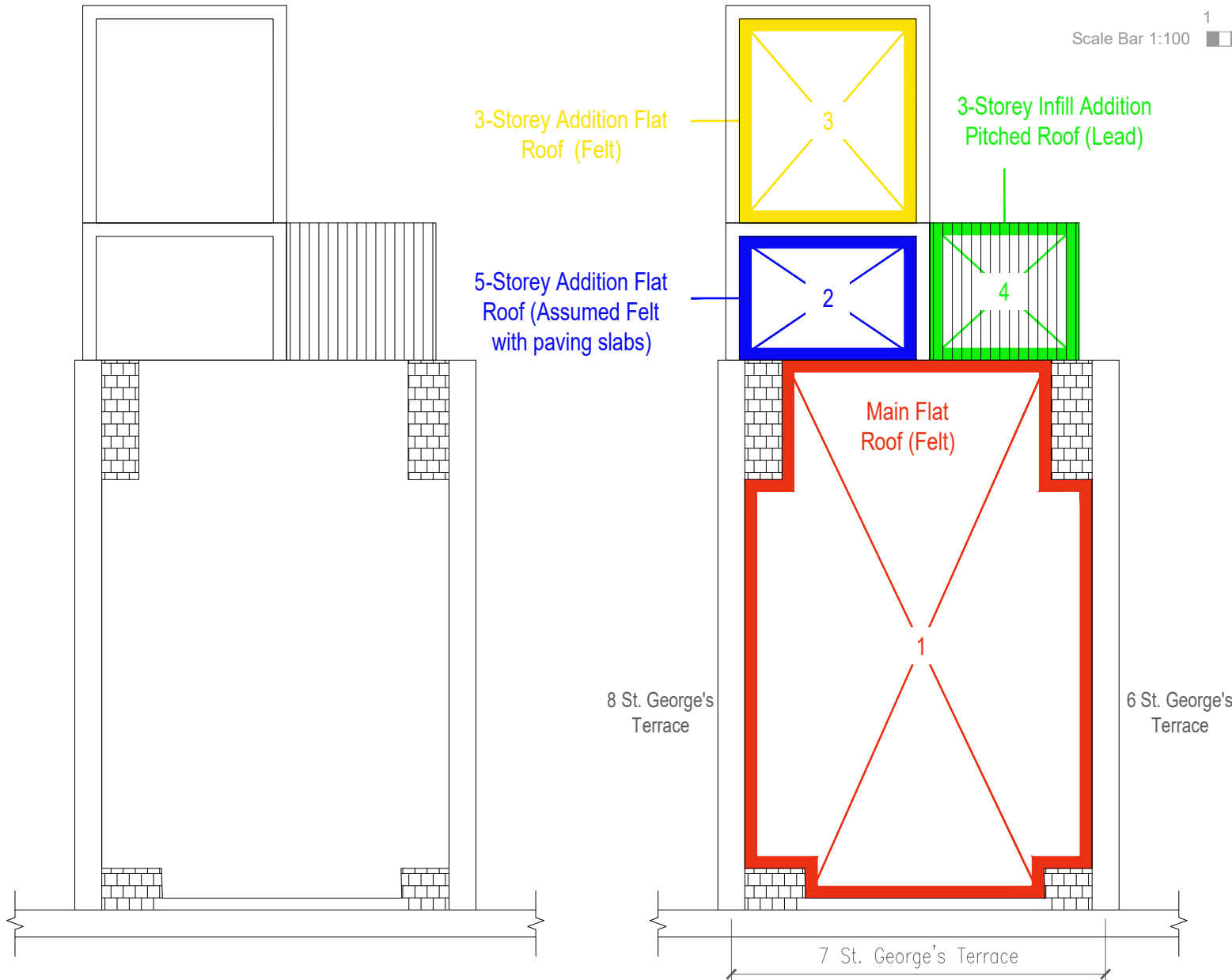
1 Existing Roof Plan Scale: 1:100 @ A4
