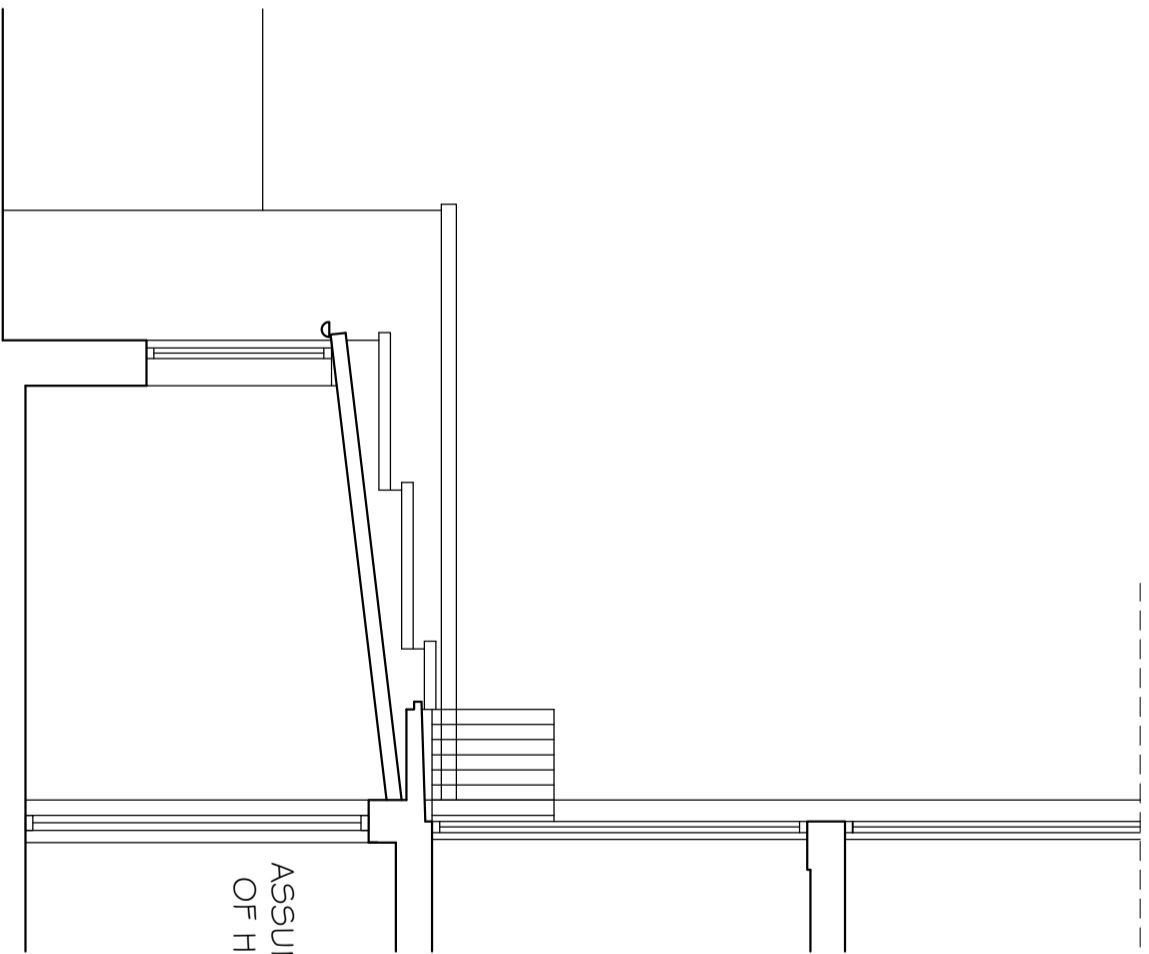
SIDE ELEVATION AS SEEN FROM NO. 11
