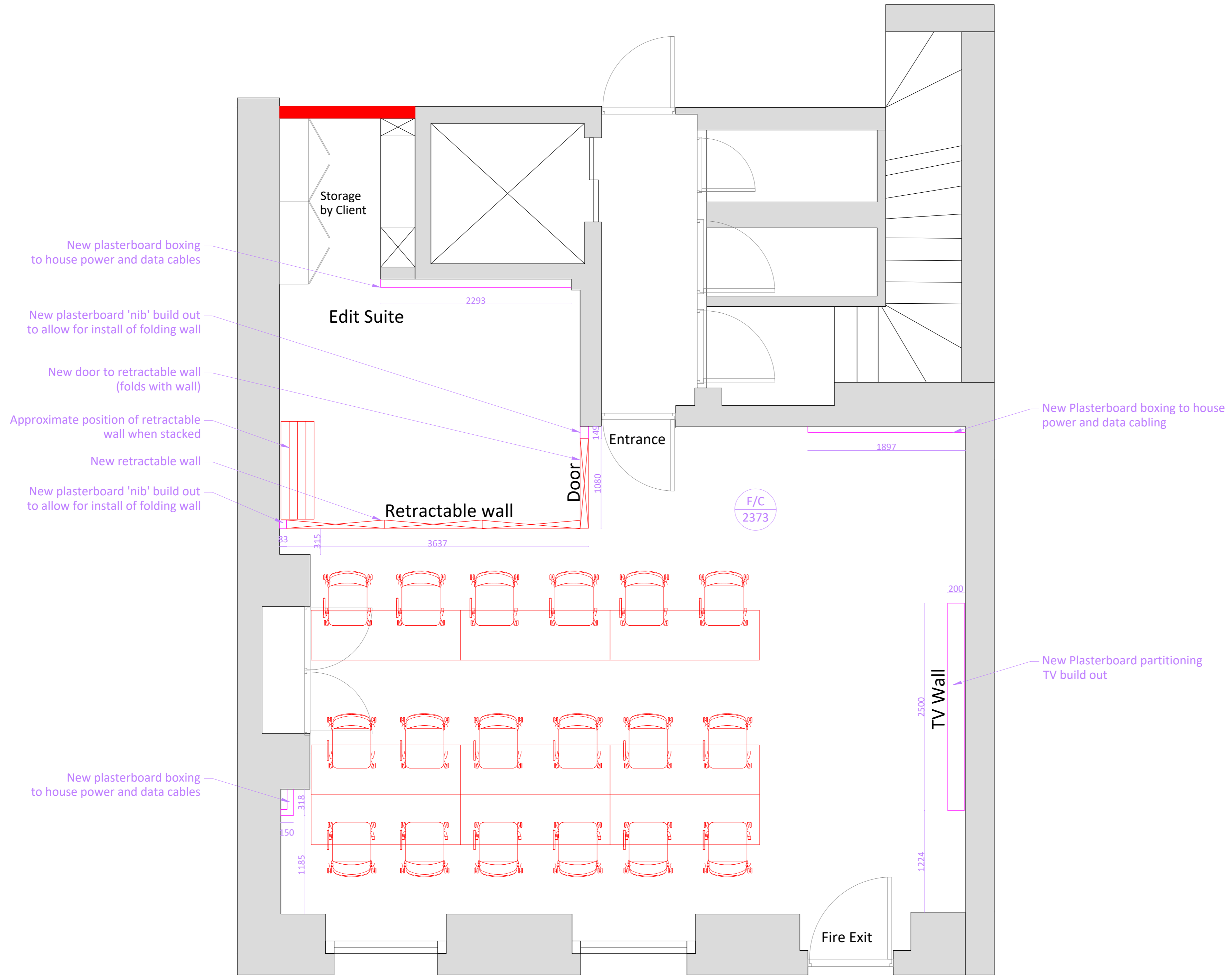
PLAN VIEW
